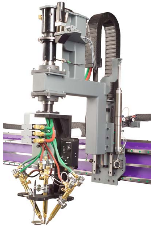
Infinite Rotation Oxyfuel Triple Bevel Head
