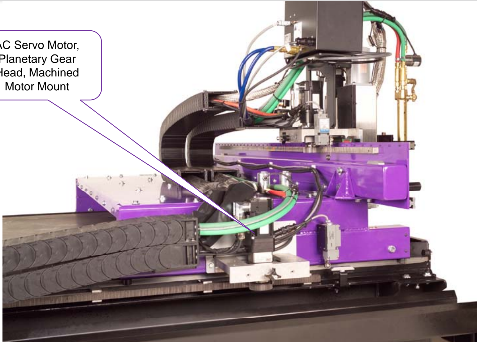
Main Rail and View of Back Deck
