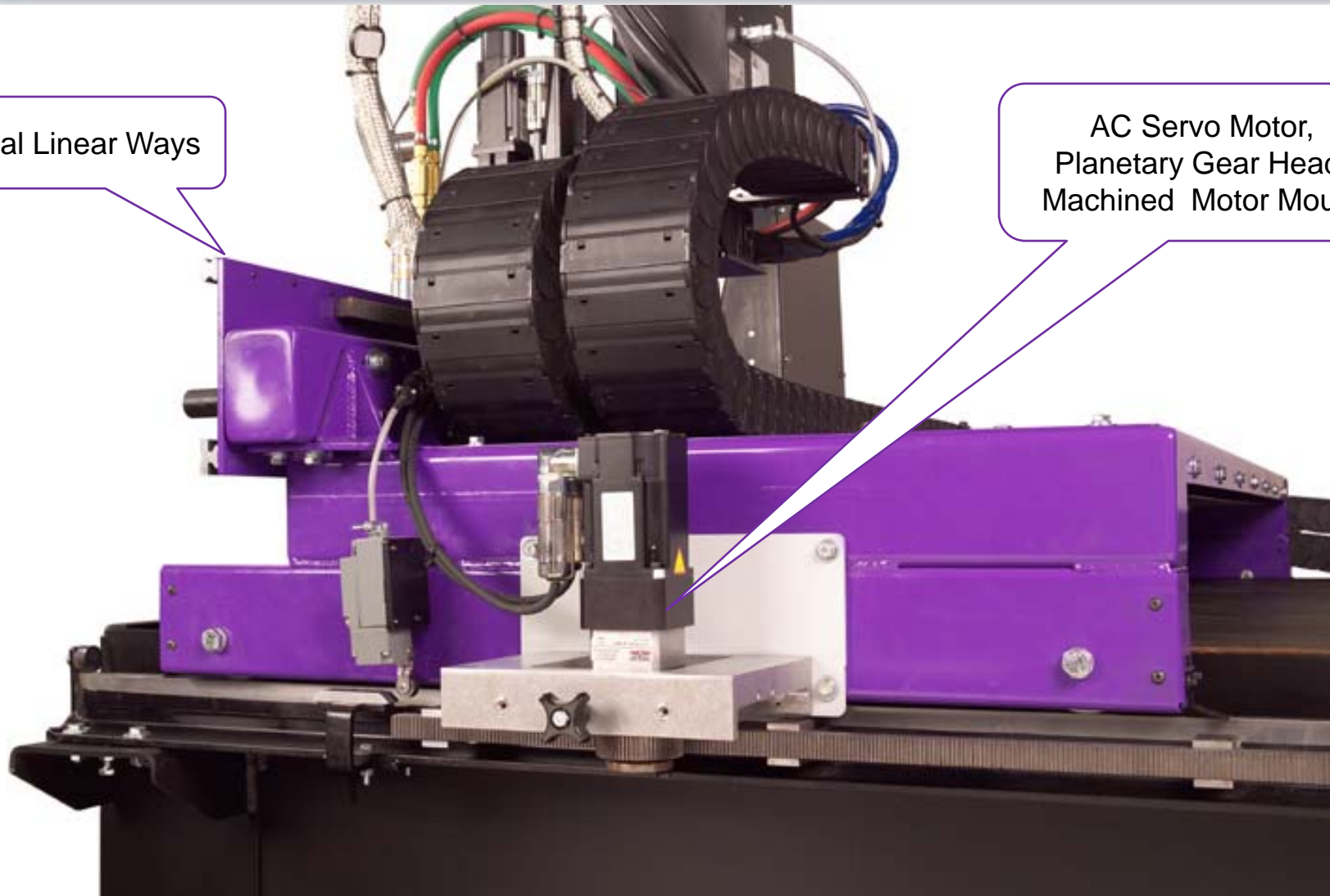
Outboard Side Rail and View of Back Deck
