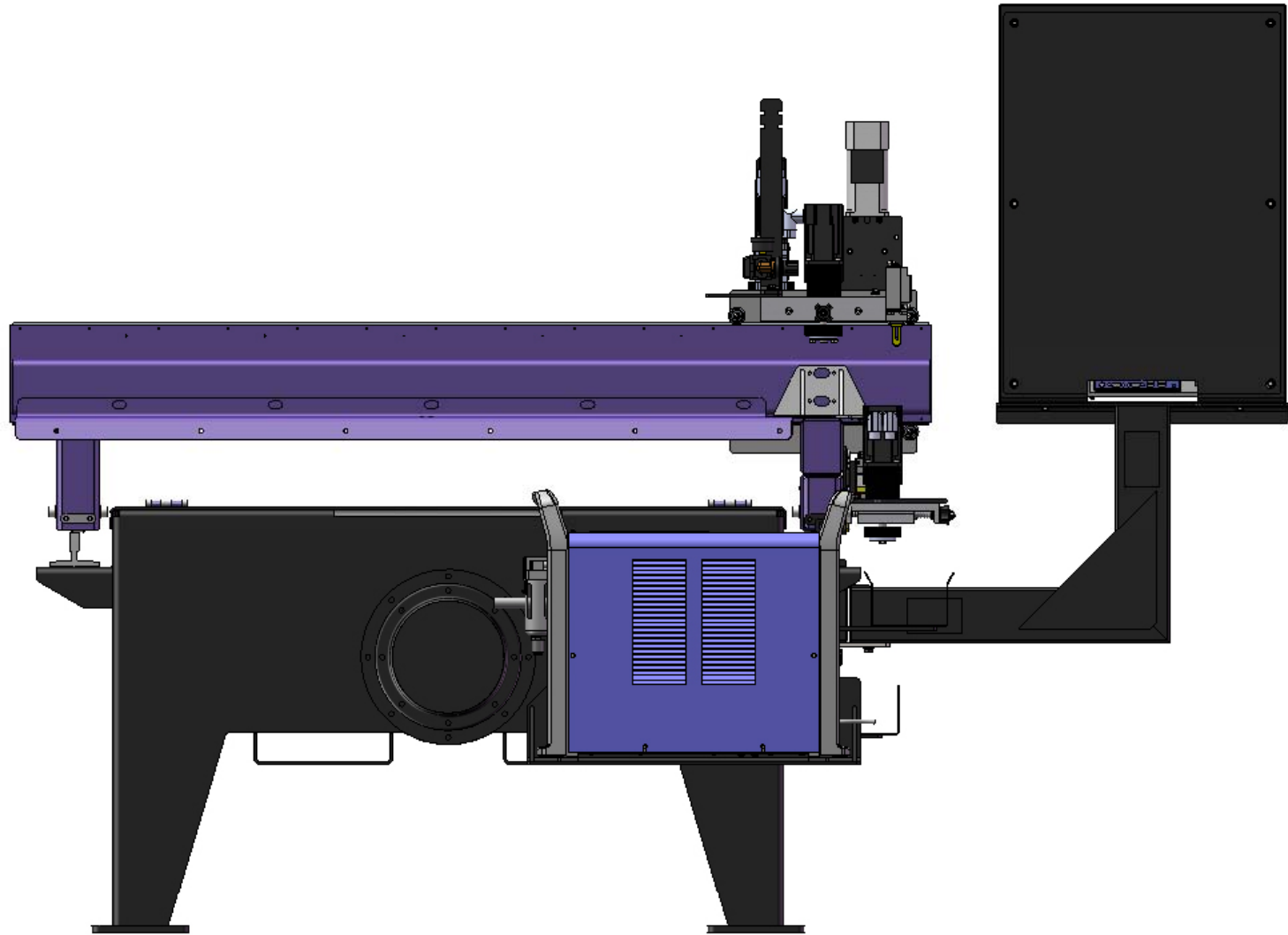
10" Air exhaust flange and plasma power supply mounting
