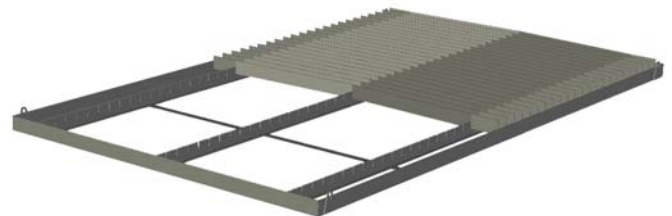
Removable Slat Sections with individual slats. Assembly also includes an expanded metal layer to catch parts that fall through the slats. - not shown in this image.
