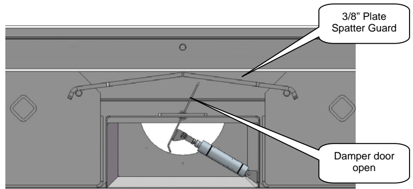
End view of air table showing exhaust tunnel and air cylinder activated damper door in the open position.
