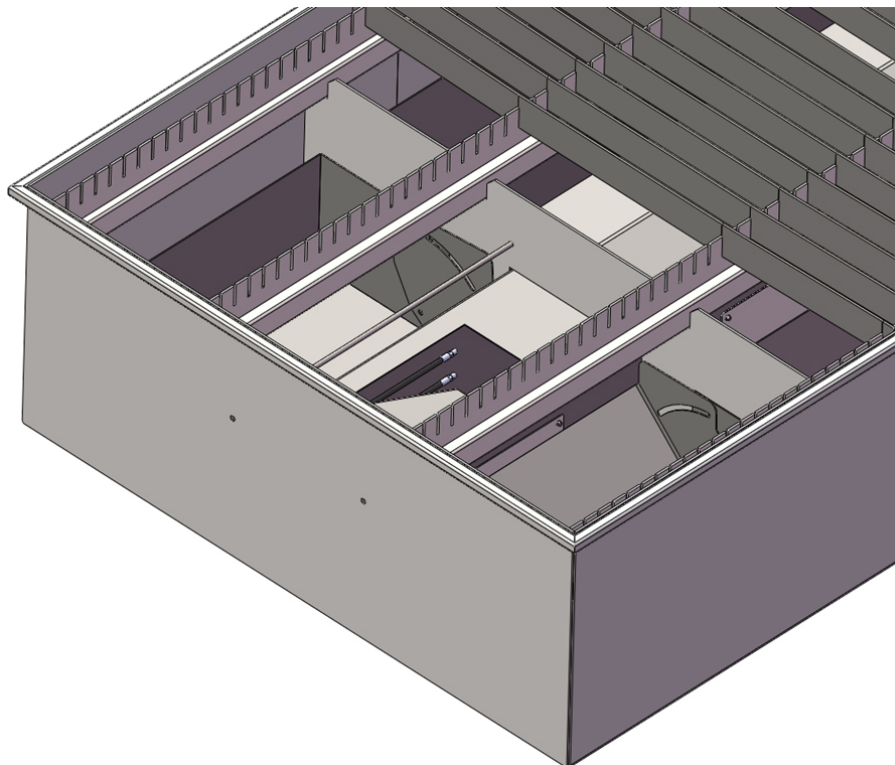
Blast shield and slats have been removed to expose the center exhaust tube and air cylinder activated damper door.
