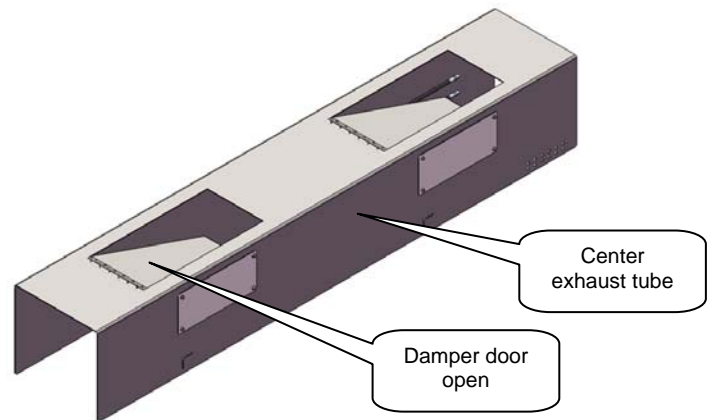
Side view of air table center exhaust tube showing an open damper door.
