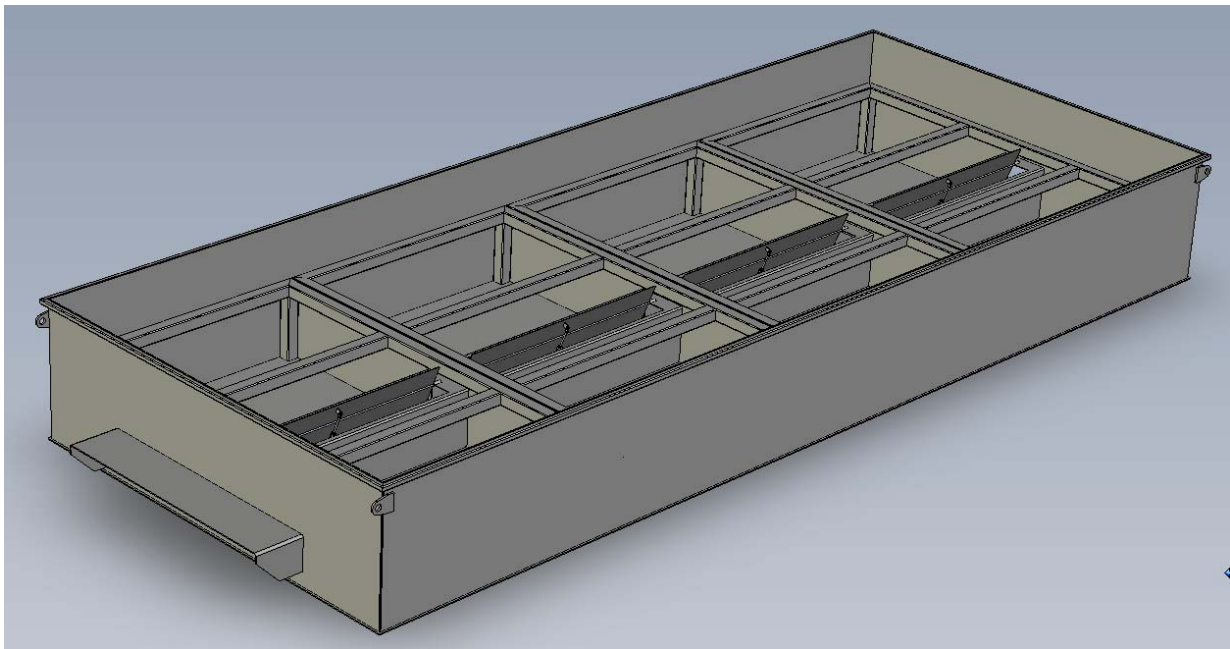
Four Zones of Air Table - Slag Trays removed to expose center air tube and air cylinder activated dampers
