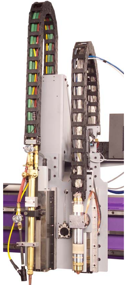
Motorized oxy-fuel station (at left) with optional Victor MT318 machine torch and auto ignition
